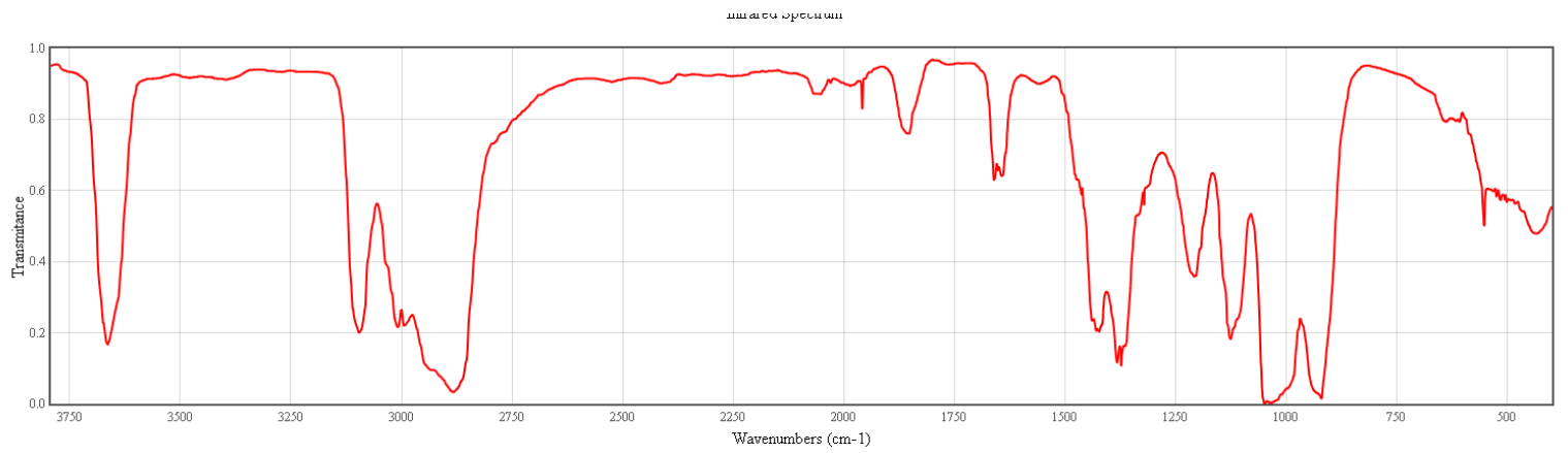
IR-A5 C 3 H 6 O (gas phase spectrum)
